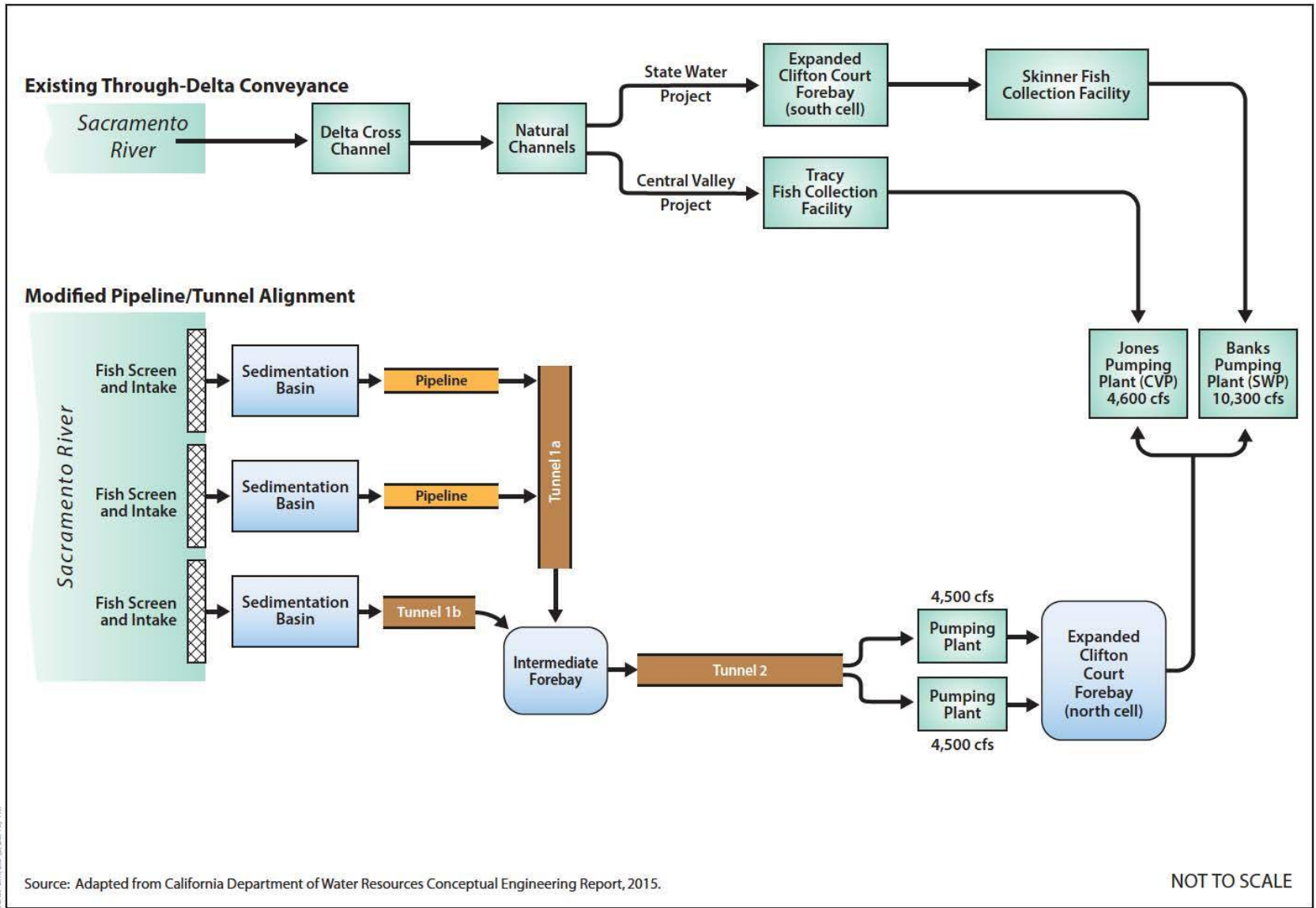
Figure 3-10 Alternatives 4 and 4A Conveyance Schematic
